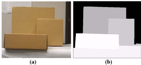
Figure 10: Usefulness of signed edge matching in low contrast scenes. (a) Left view. (b) Disparity map obtained by using belief propagation with matching costs including signed edge matching. This allows us to handle low-contrast scenes, where depth discontinuities may not correspond to intensity edges .
