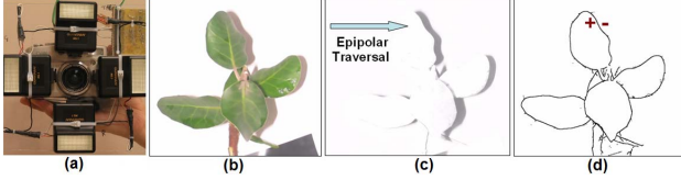
Figure 1: (a) Multi-flash camera (b) Image taken with left flash. (c) Correspondent ratio image and traversal direction. (d) Computed depth edges. Note that we can obtain the sign of each depth edge pixel, indicating which side of the edge is the foreground.
