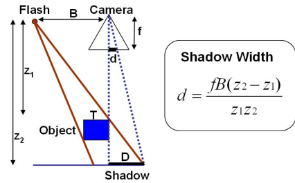
Figure 3: Relationship of shadows and relative depth.
